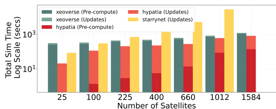
Fig. 3: The total simulation time (including pre-compute and simulation updates times) for the 3 simulators when varying the number of satellites from 25 to 1584. xeoaverse 's simulation update time is 2.3x and 40x times less than Hypatia and StarryNet , respectively.
