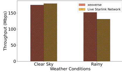
Fig. 6: xeoerse captures the impact of weather conditions on the downlink throughput in the bent-pipe connection for Starlink user terminal. xeoerse shows results that are close to reality: within 2% for clear sky and within 16% for rainy conditions.
