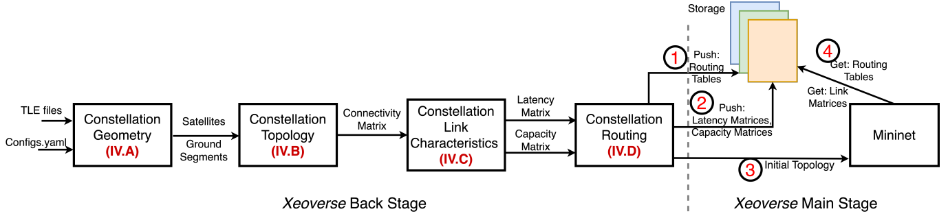
Fig. 1: Workflow of xeoVerse Simulator. The process is divided into two stages. The xeoVerse Back Stage builds the constellation topology, calculate the link characteristics in terms of latency and capacity, and finally compute the routing tables for each satellite. The xeoVerse Main Stage configures a Mininet topology based on the inputs from xeoVerse Back Stage, and run applications on top of Mininet.
